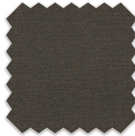
R-127 - MOONROCK
